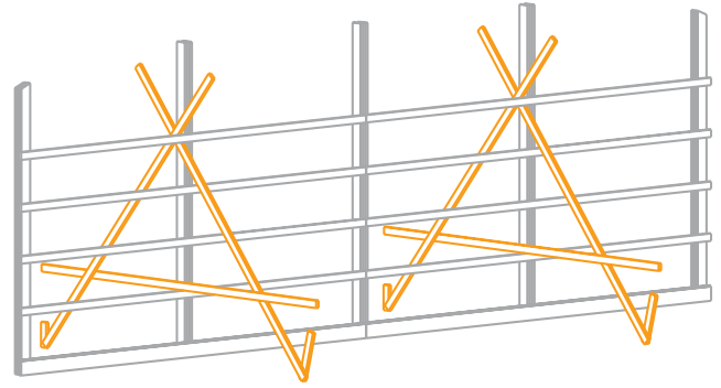
A-Frame Ground Bracing Perpendicular to the Wall
