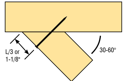
FIGURE B8-10 Corner jack to corner Girder Truss
