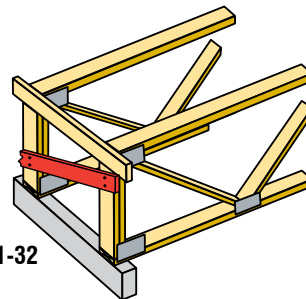
Ribbon board with Diagonal Brace
