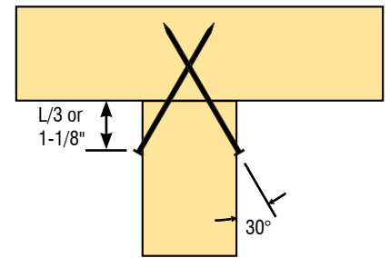
FIGURE B8-9 End jack to hip Girder Truss
