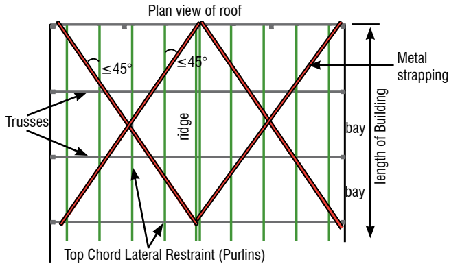
FIGURE B10-21 Bracing of Top Chords using Metal Strap Cross Bracing
