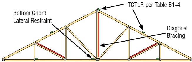
Apply Diagonal Bracing to Webs that are near the Bottom Chord Lateral Restraint. See "IMPORTANT NOTE" on page 14 for spacing of Bottom Chord Lateral Restraint.
