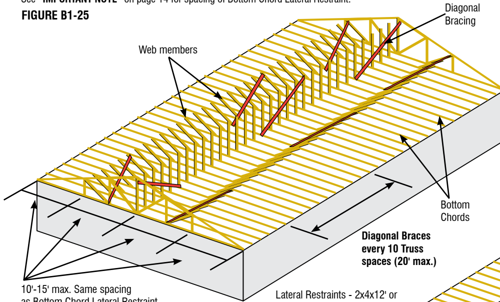
Apply Diagonal Bracing to Webs that are near the Bottom Chord Lateral Restraint. See "IMPORTANT NOTE" on page 14 for spacing of Bottom Chord Lateral Restraint.
