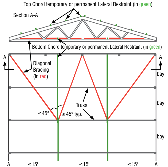
FIGURE B10-19 Bottom Chord Restraint and Bracing
