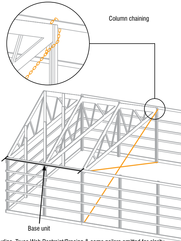
Purlins, Truss Web Restraint/Bracing & some nailers omitted for clarity. See Step 3 for Temporary Restraint & Bracing requirements for the Trusses.
