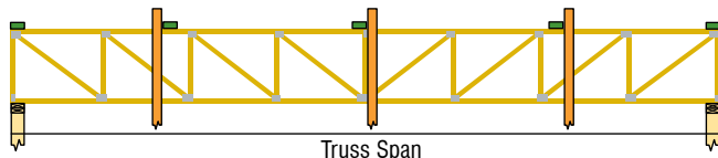
Parallel Chord roof Truss with Top Chord Temporary Lateral Restraint and Ground Brace verticals.
