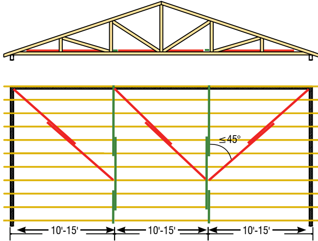
Plan view of Bottom Chord Lateral Restraint and Diagonal Bracing. Top Chord and Web Lateral Restraint and Diagonal Bracing not shown for clarity.
