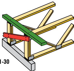
Top Chord Temporary Lateral Restraint with Diagonal Brace
